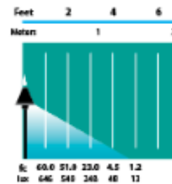
AL-18-SM Half Spread Photometrics 12ft (3.7m) diameter
